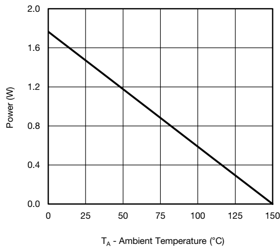
Power Junction to Ambient
